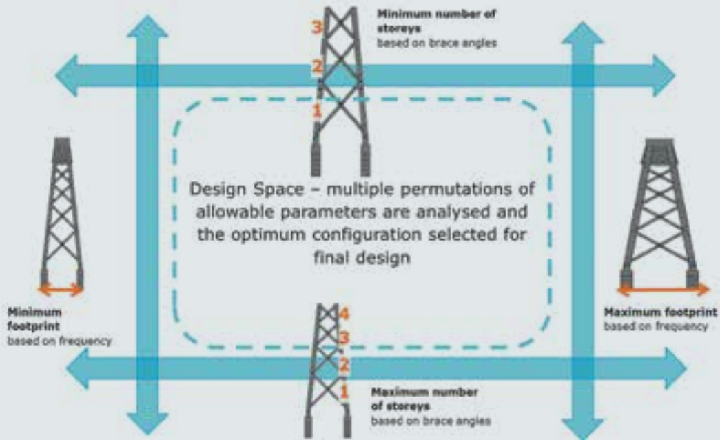
FIGURE 8-7: JACKET MODEL OVERVIEW
