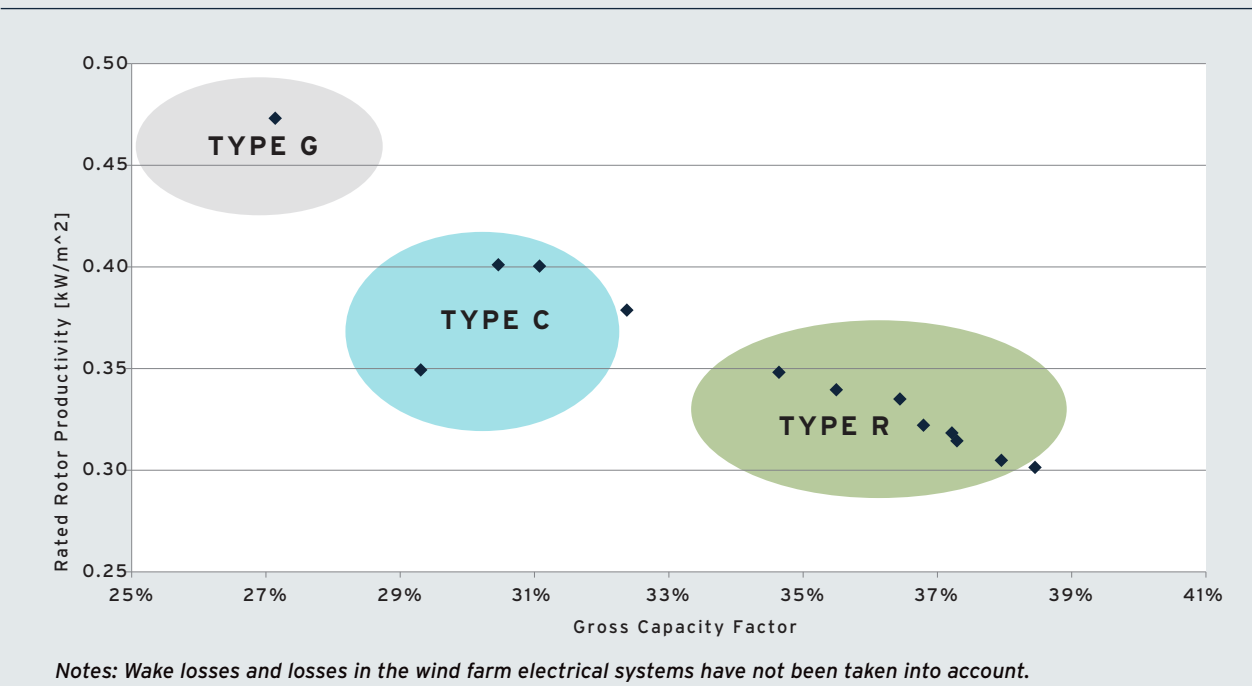
FIGURE 6-3: WIND TURBINE GROSS CAPACITY FACTOR AGAINST RATED ROTOR PRODUCTIVITY (7.9 M/S MEAN ANNUAL WIND SPEED AT 100 M MSL)
