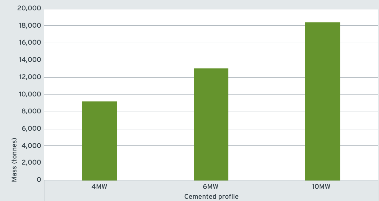
FIGURE 8-9: GBS ON SEABED MASS
