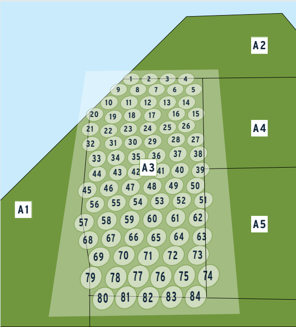
FIGURE 7-2: TAMIL NADU SUB ZONE A3 504MW 6MW OFFSHORE WINDFARM LAYOUT
