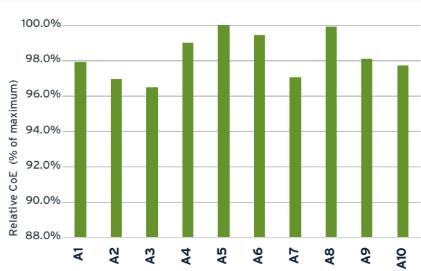
FIGURE 4-4: SPATIAL ANALYSIS RESULTS: COST OF ENERGY RELATIVE TO MAXIMUM OF SUB-ZONES
