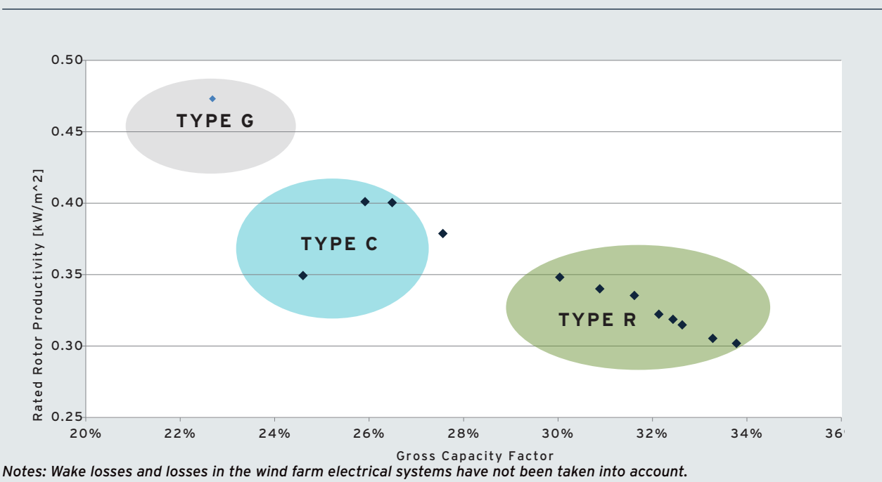
FIGURE 6-4: WIND TURBINE GROSS CAPACITY FACTOR AGAINST RATED ROTOR PRODUCTIVITY (7.8 M/S MEAN ANNUAL WIND SPEED AT 80 M MSL)
