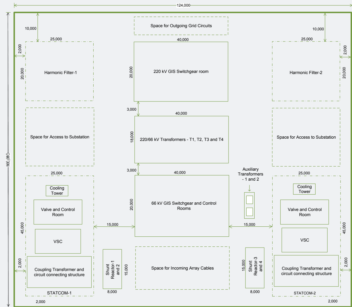
FIGURE 8-4: ONSHORE SUBSTATION LAYOUT
