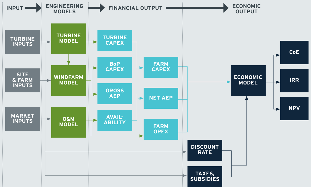
FIGURE 10-1: TURBINE.ARCHITECT PROCESS
