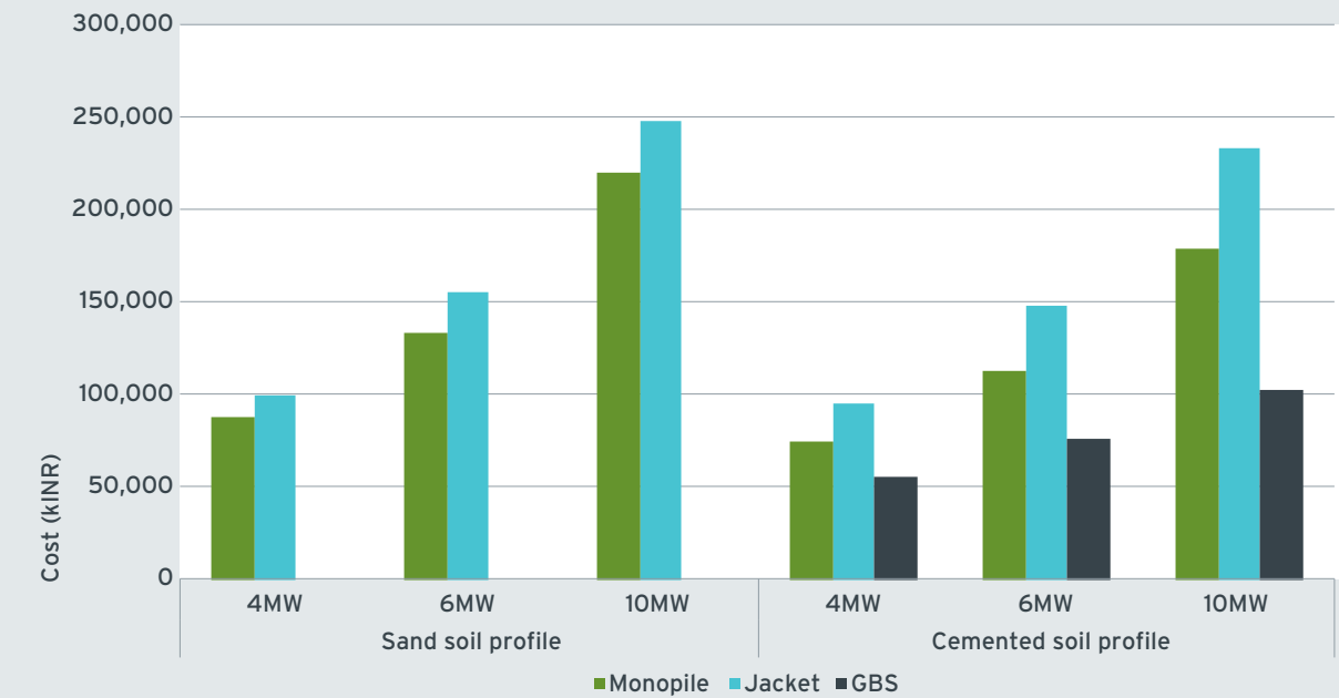
FIGURE 8-10: SUPPORT STRUCTURE COST COMPARISON
