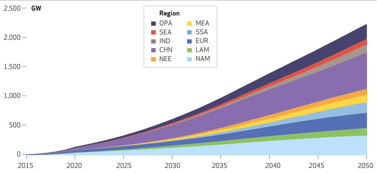
FIGURE 10: FORECAST OF OFFSHORE WIND CAPACITY BY REGION (DNV GL ETO)
