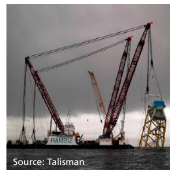
Figure 76 - Rambiz up-ending the leg-sheered jacket at Beatrice
