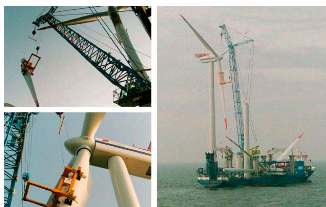
Figure 64 - A2Sea Sea Energy / Sea Power - Leg-stabilised crane vessels
