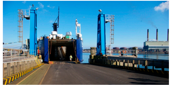
Figure 93 - 180 tonne RoRo linkspan
