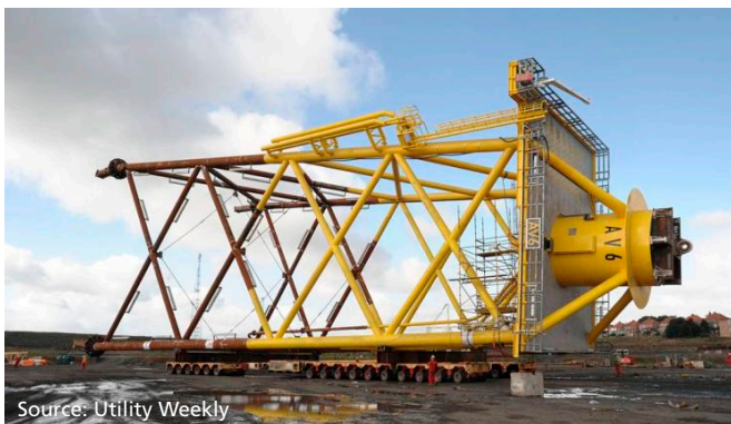
Figure 42 - Jacket transportation on the quay
