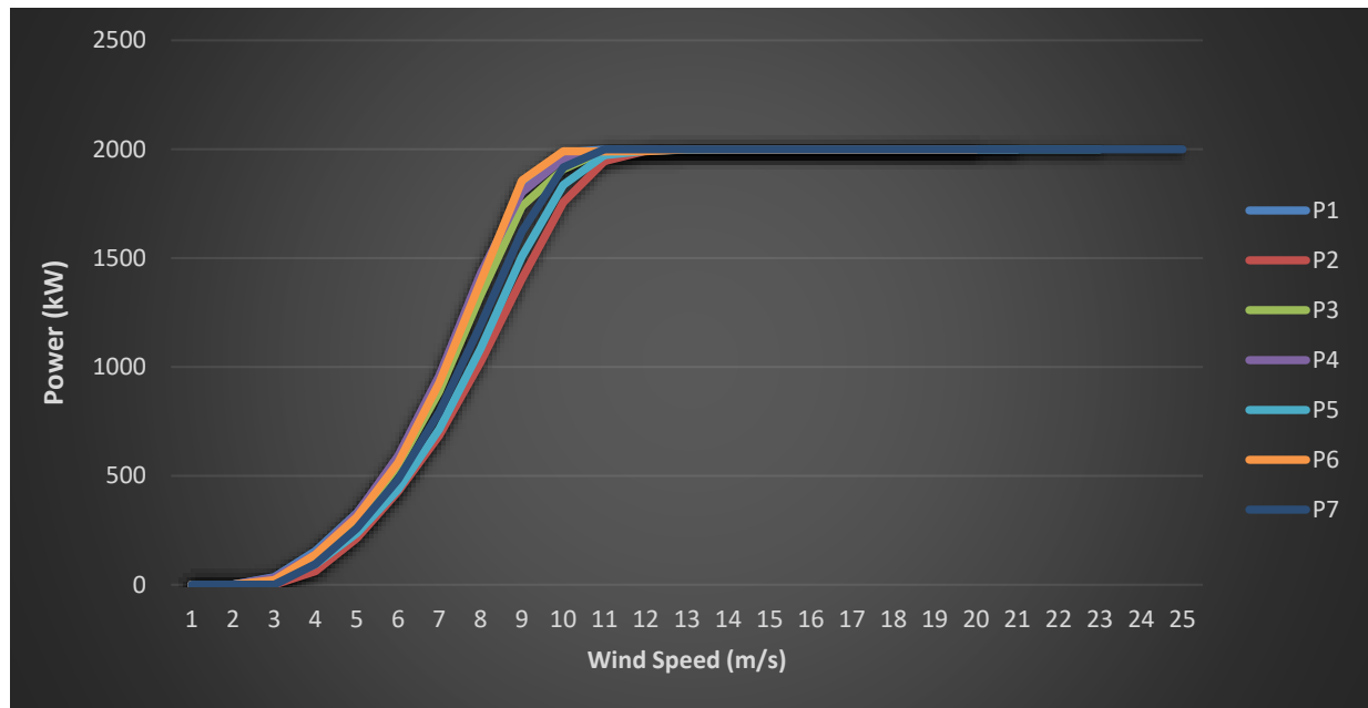
Figure 7: Power Curves considered for the study
