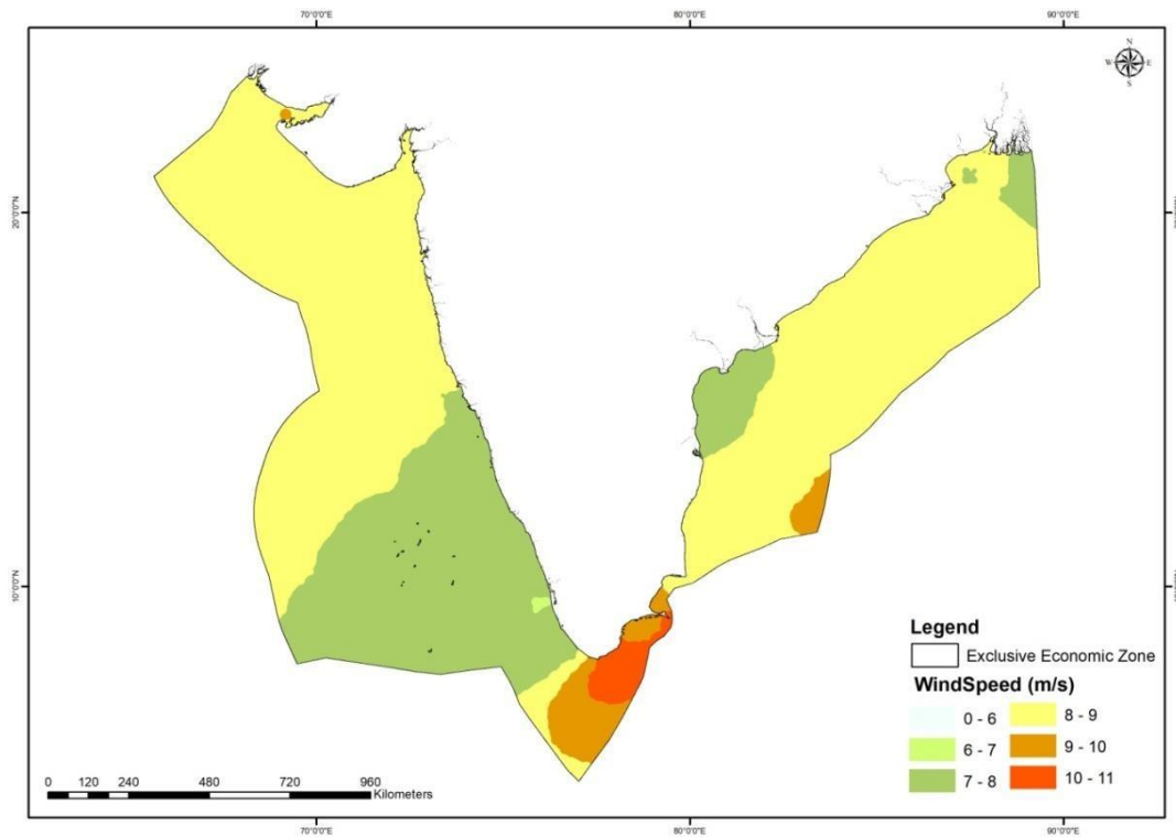
Figure 13: Offshore Wind speed map up to EEZ at 120m amsl
