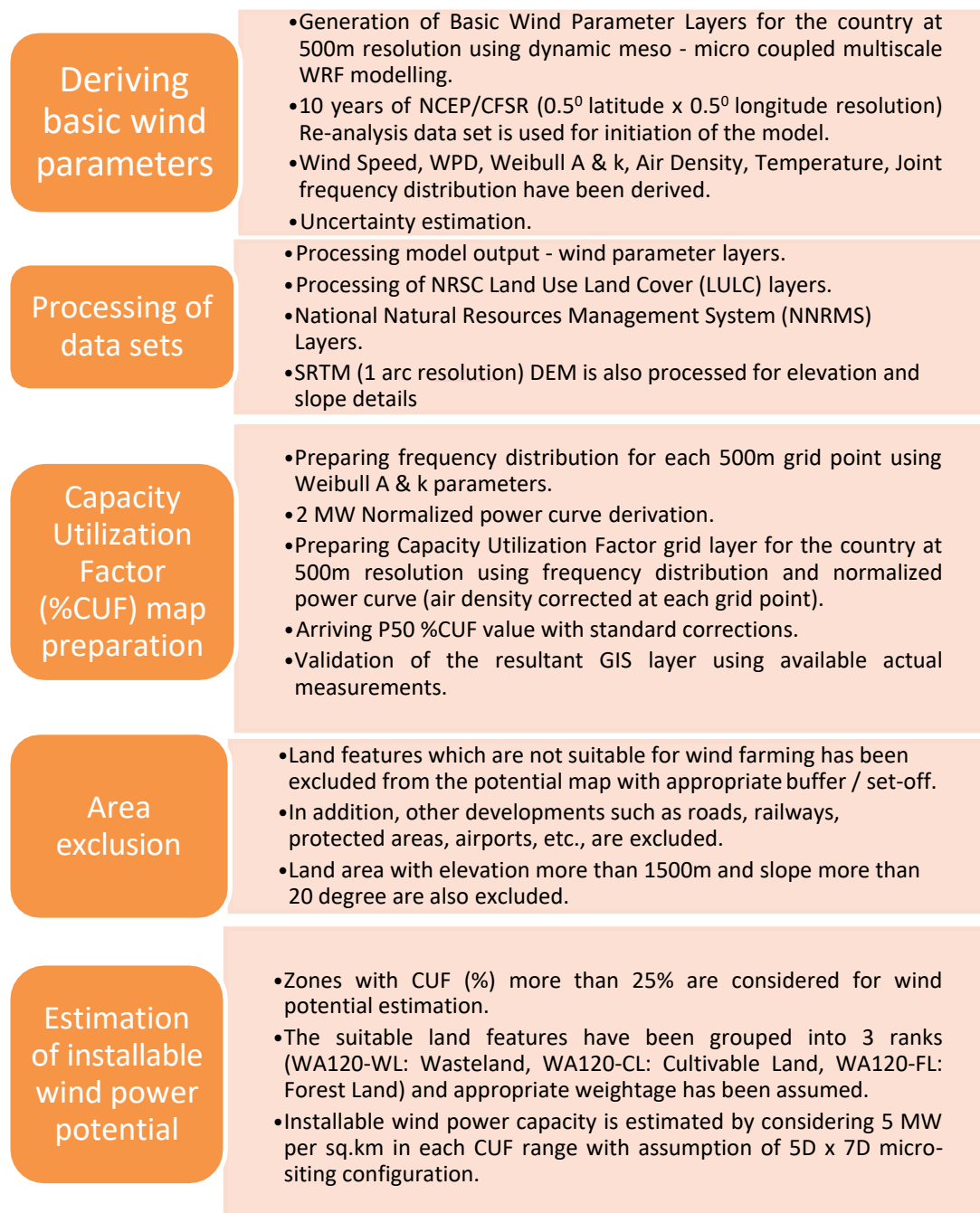
Figure 6: Outline of the Methodology
