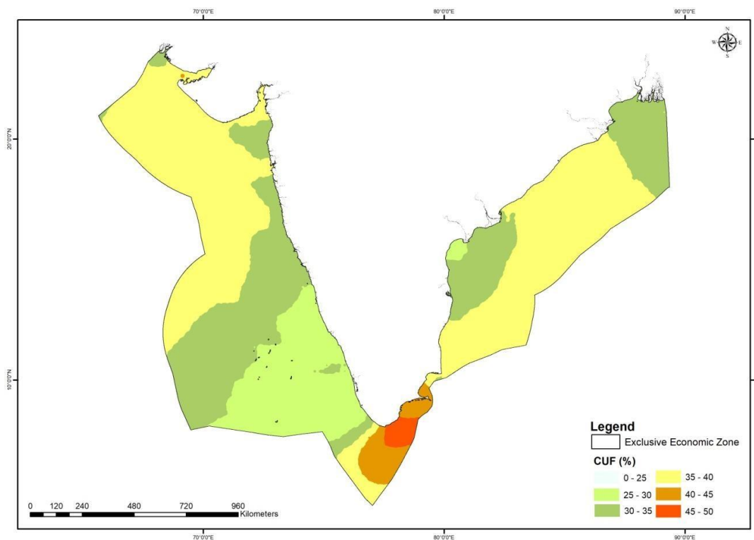
Figure 14: Offshore Wind Power Potential Map up to EEZ at 120m amsl
