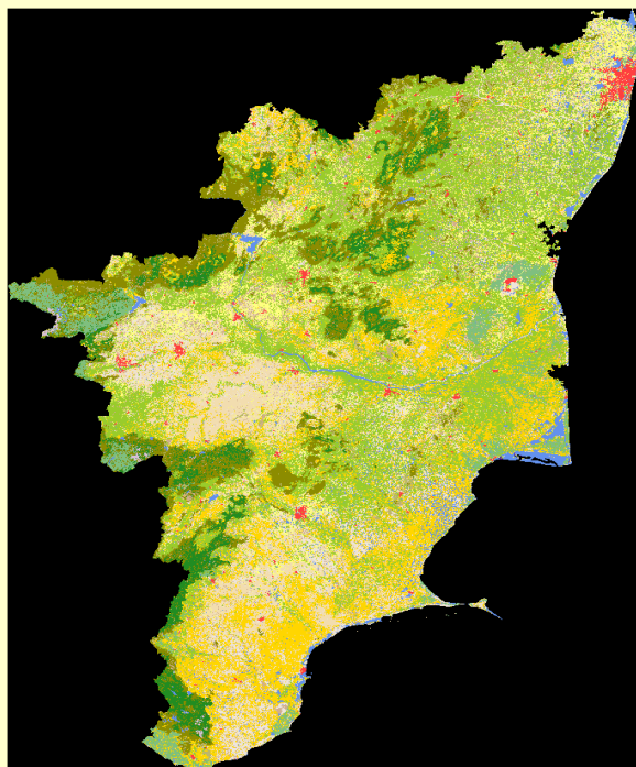
Figure A.2 RSC LULC (Land Use Land Cover) Sample for Tamil Nadu
