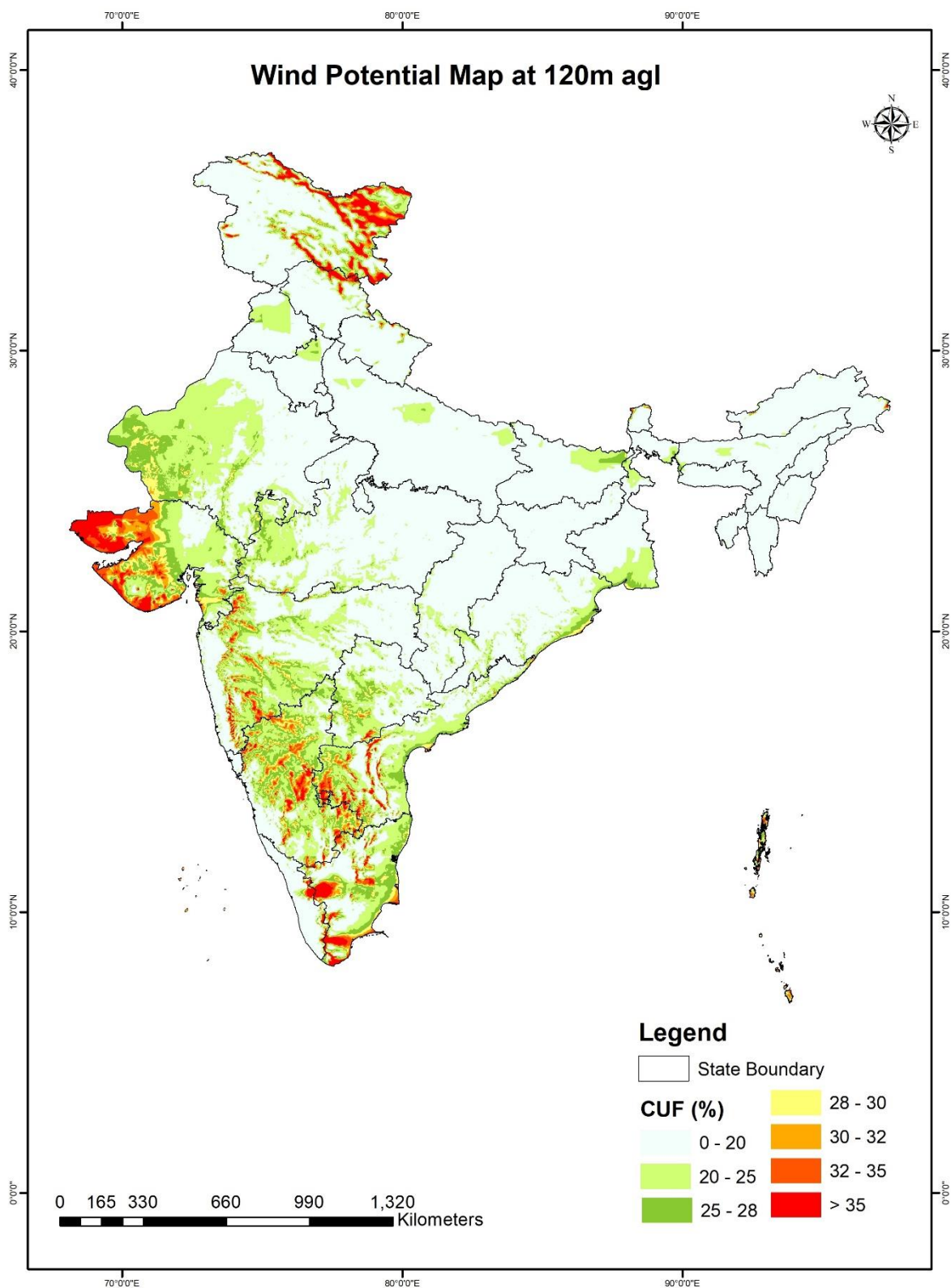
Figure 9: Wind Potential Map of India at 120m agl
