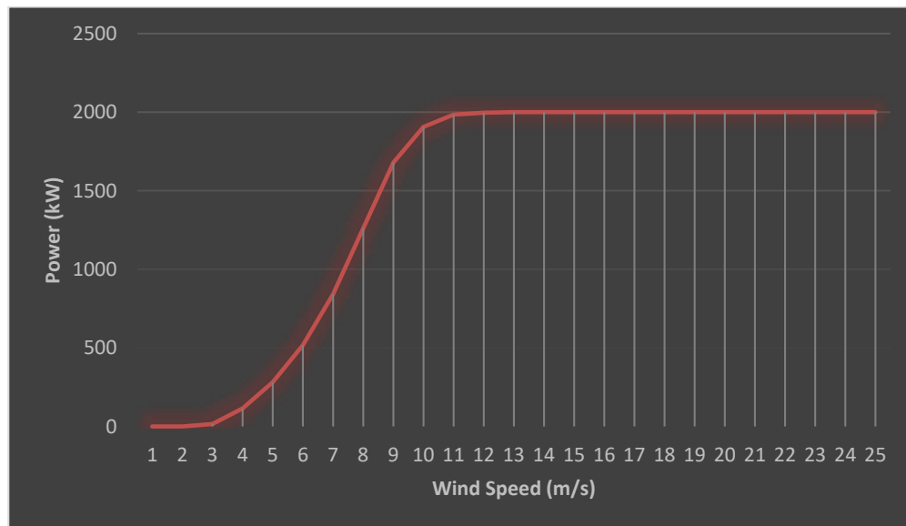
Figure 8: Normalized Power Curve
