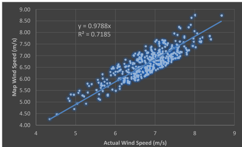
Figure 12: Scatter Plot showing the comparison between Estimated and Actual Wind Speed for 406 stations
