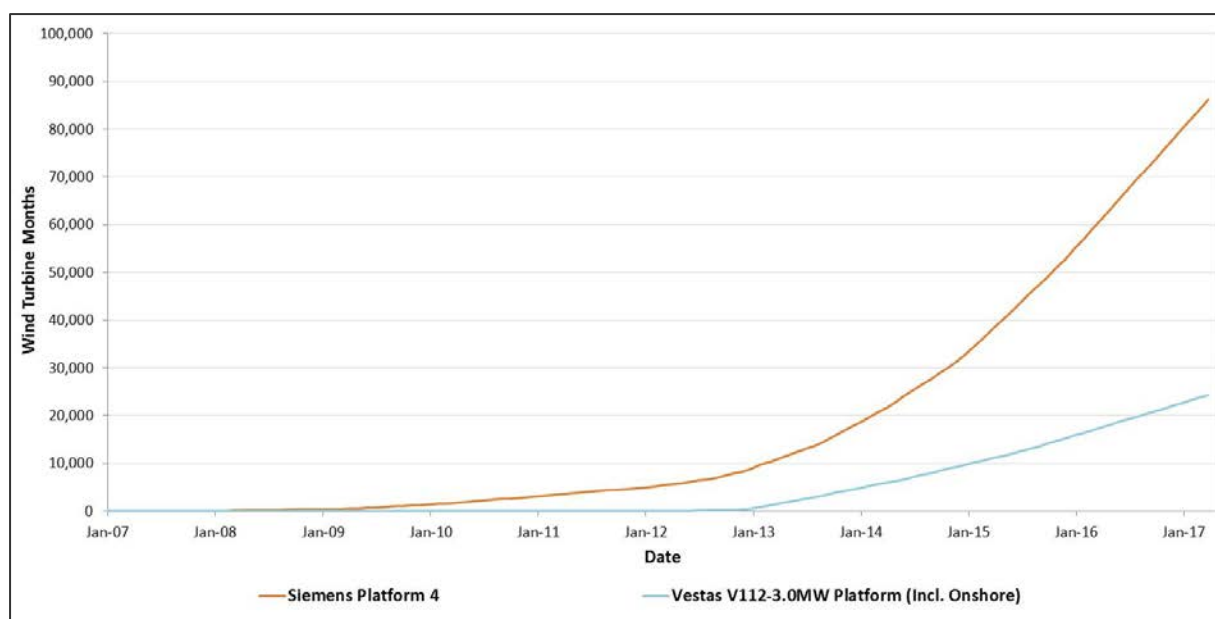
Figure 9: Offshore platform track records in wind turbine operating months (Siemens and Vestas examples).
