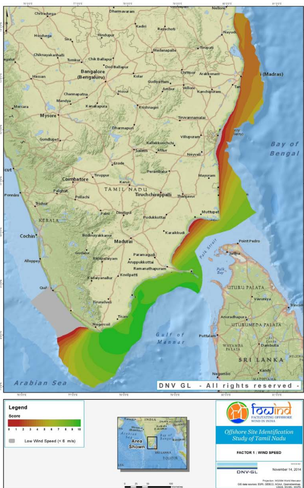
Figure 38: Offshore Wind Speed Heat Map Tamil Nadu.
