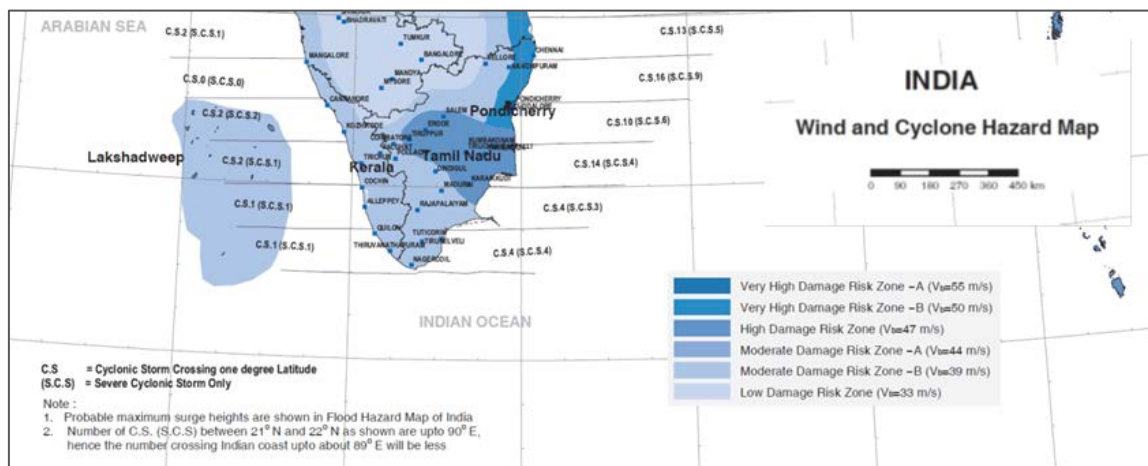
Figure 5: Wind and Cyclone Hazard Zones & the Basic Wind Speed in Tamil Nadu Source: [21]
