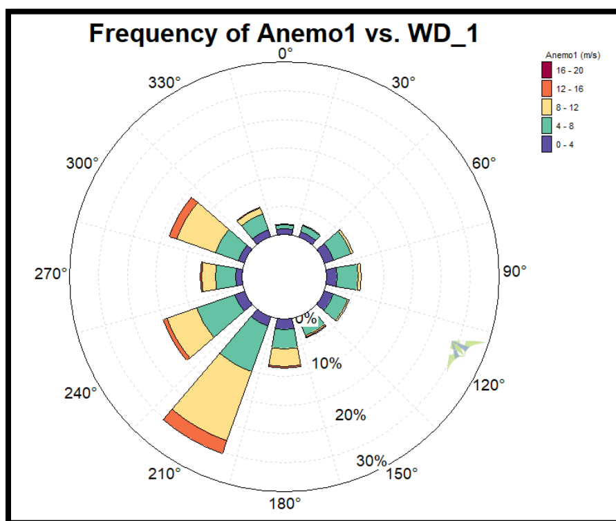
Figure 10: Wind Rose
