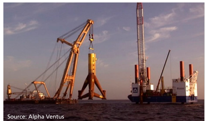
Figure 60 - Sheerleg crane-vessel working in tandem with a jack-up piling vessel
