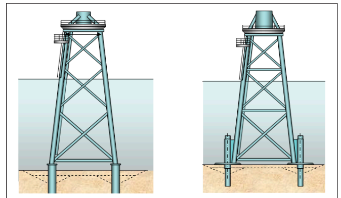
Figure 71 - Wind turbine substructure concept - jacket (pre-piled & post-piled)
