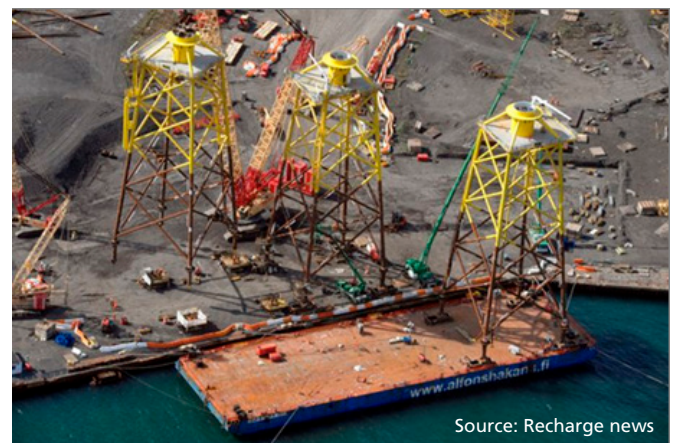
Figure 44 - Jacket load-out onto deck barges
