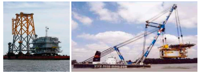
Figure 81 - Barge for transport and SHLV for installation of OSS foundation and topside
