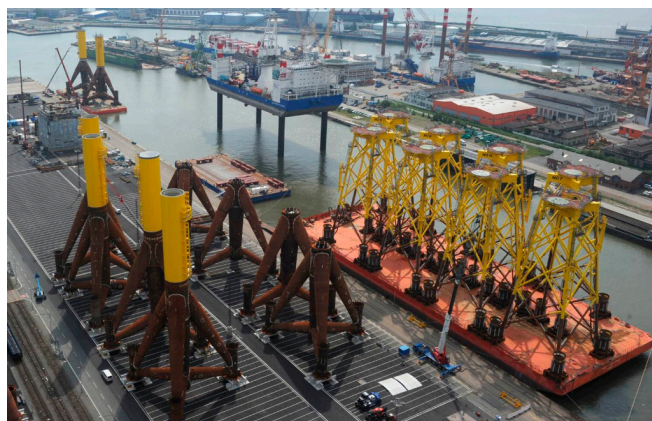
Figure 19 - Port of Bremerhaven (Germany) - WTG foundation fabrication
