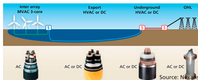
Figure 13 - Offshore wind export and array cable types
