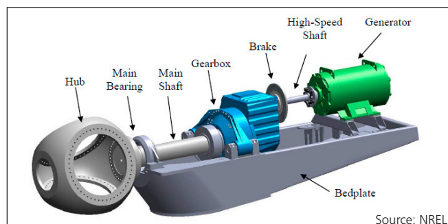
Figure 9 - WTG modular drivetrain configuration
