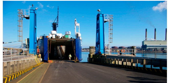
Figure 93 - 180 tonne RoRo linkspan
