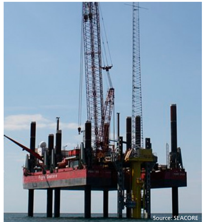
Figure 2 - Offshore met mast installation, UK
