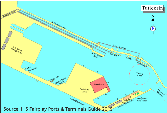
Figure 130 - Tuticorin port estate
