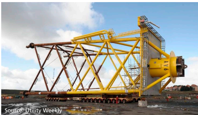
Figure 42 - Jacket transportation on the quay
