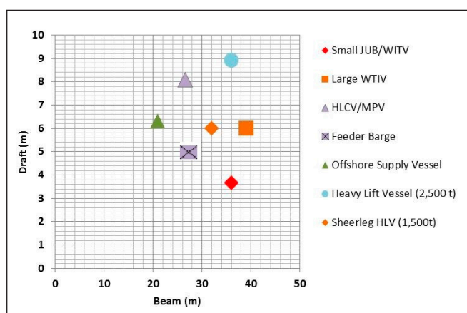
Figure 67 - Vessel port access requirement chart for example vessels
