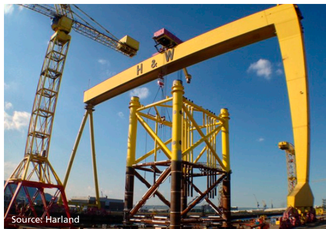
Figure 48 - Offshore substation jacket foundation and topside
