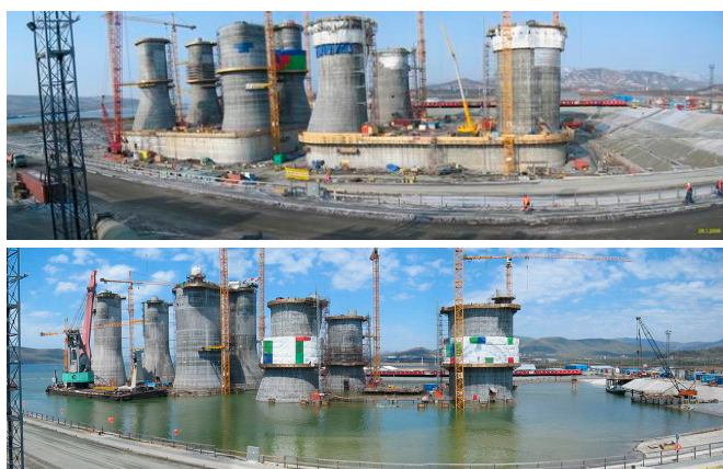
Figure 47 - GBS construction in a dry-dock facility (or graving yard)
