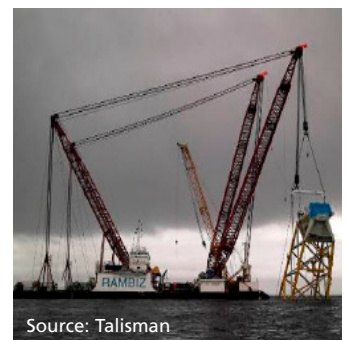
Figure 76 - Rambiz up-ending the leg-sheered jacket at Beatrice
