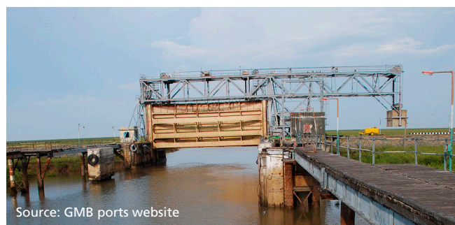
Figure 115 - Bhavnagar Port - lifting gate
