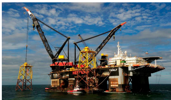
Figure 66 - Jacket installation at Alpha Ventus, by Thialf
